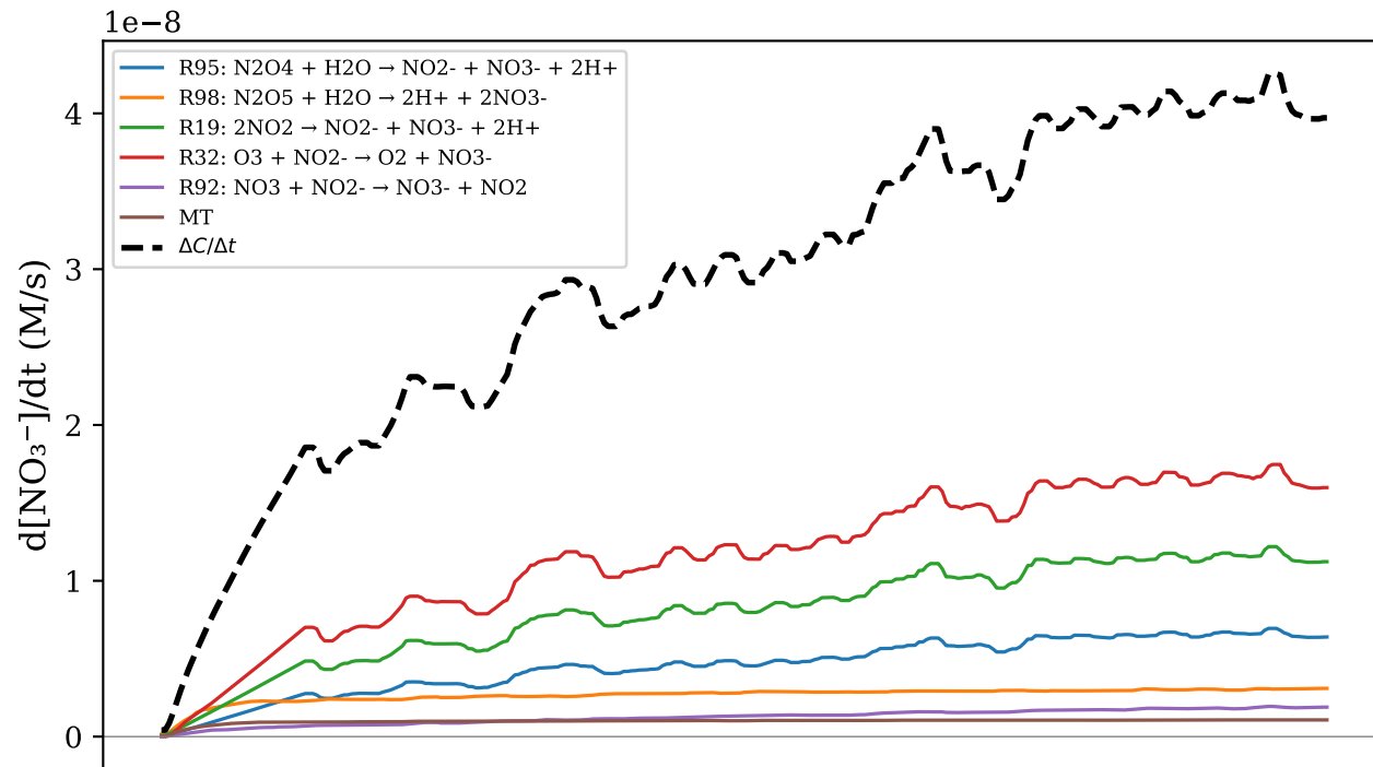
(a) \text{NO}_3^-
